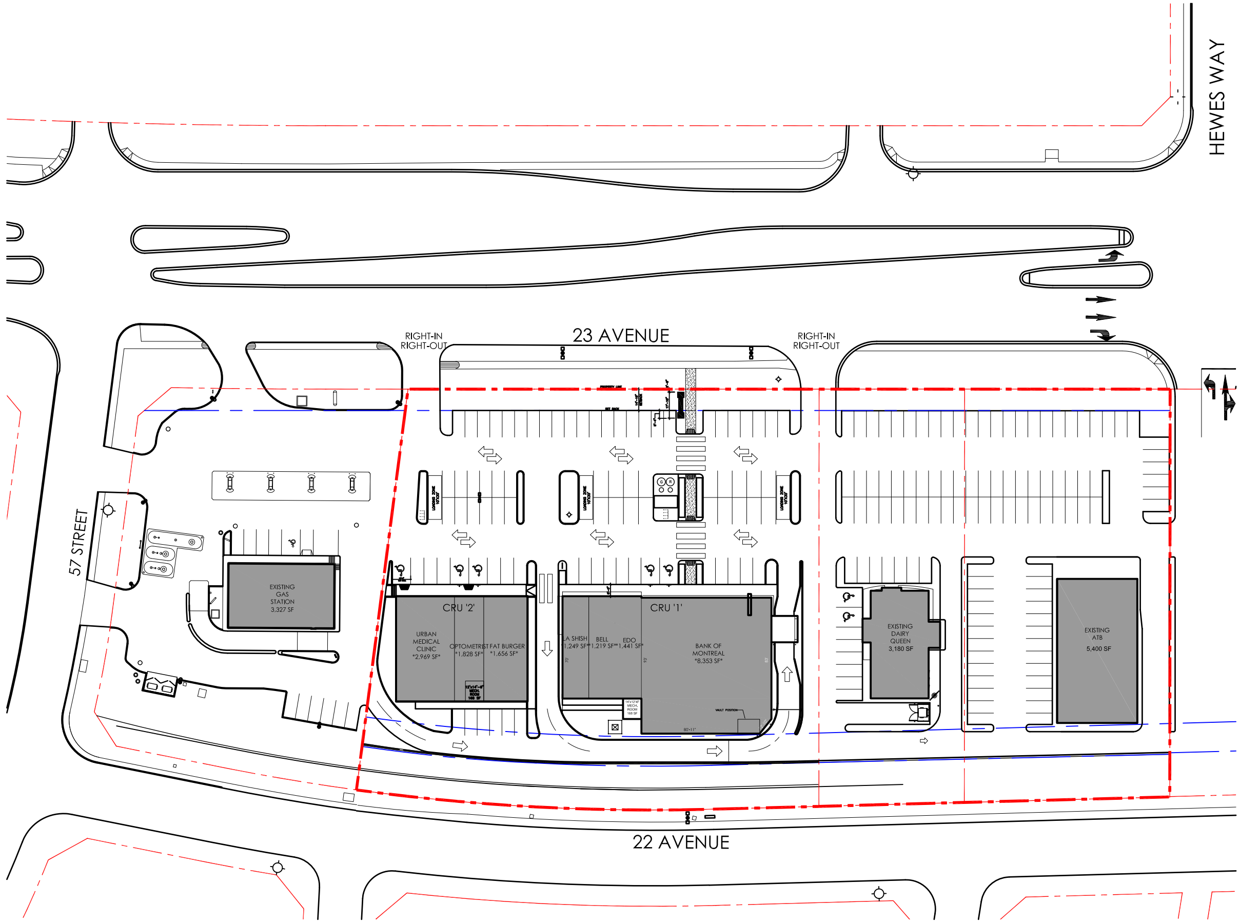
1 SITE PLAN A0-0 nts
