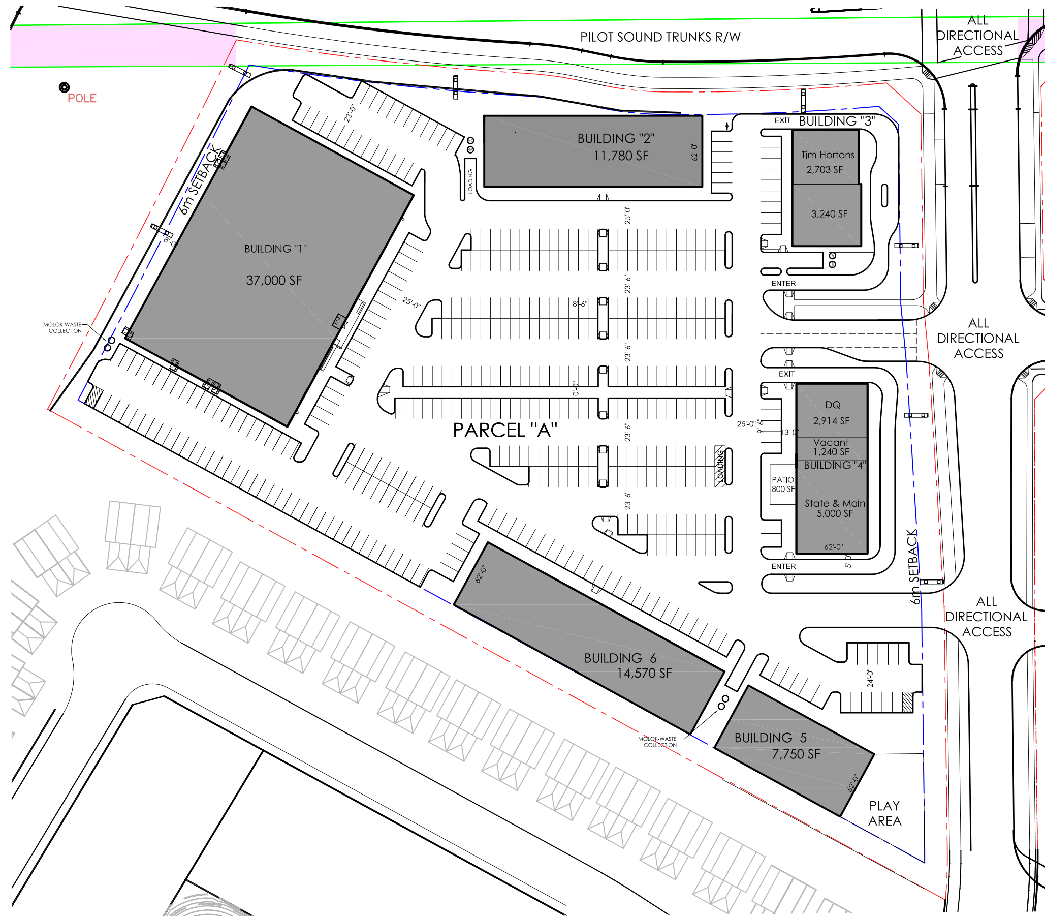
1 SITE PLAN A0-0 NTS
